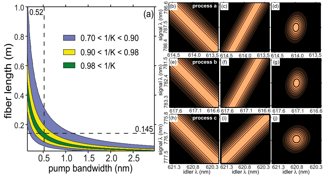
Figure 4. (a) Regions of simultaneous near-factorability for all three processes, (b–j): Plots of |\alpha(\nu_s, \nu_i)|^2 , |\phi(\nu_s, \nu_i)|^2 , and |\alpha(\nu_s, \nu_i)\phi_j(\nu_s, \nu_i)|^2 for processes a [(b–d)], b [(e–g)], and c [(h–j)].
